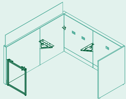
05. Support brackets
